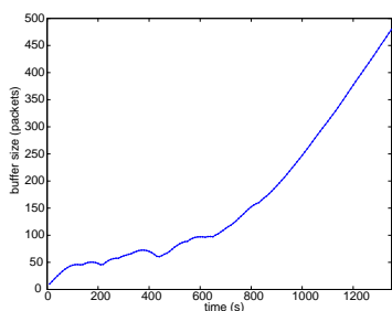
Fig. 4. Buffer size time-history as the number of active access links is increased by 1 every 20s to simulate accelerated demand growth. Algorithm parameters: target packet loss rate \lambda^* = 10^{-4} , control gain K = 2.5 , sampling interval \tau = 10s , buffer limits q_{min}=10 packets, q_{max}=500 packets. Network topology as shown in Figure 3.
